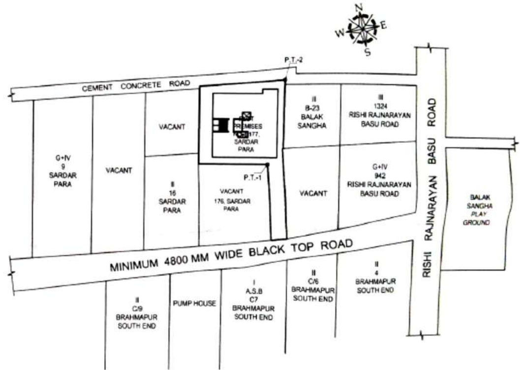
SITE PLAN
